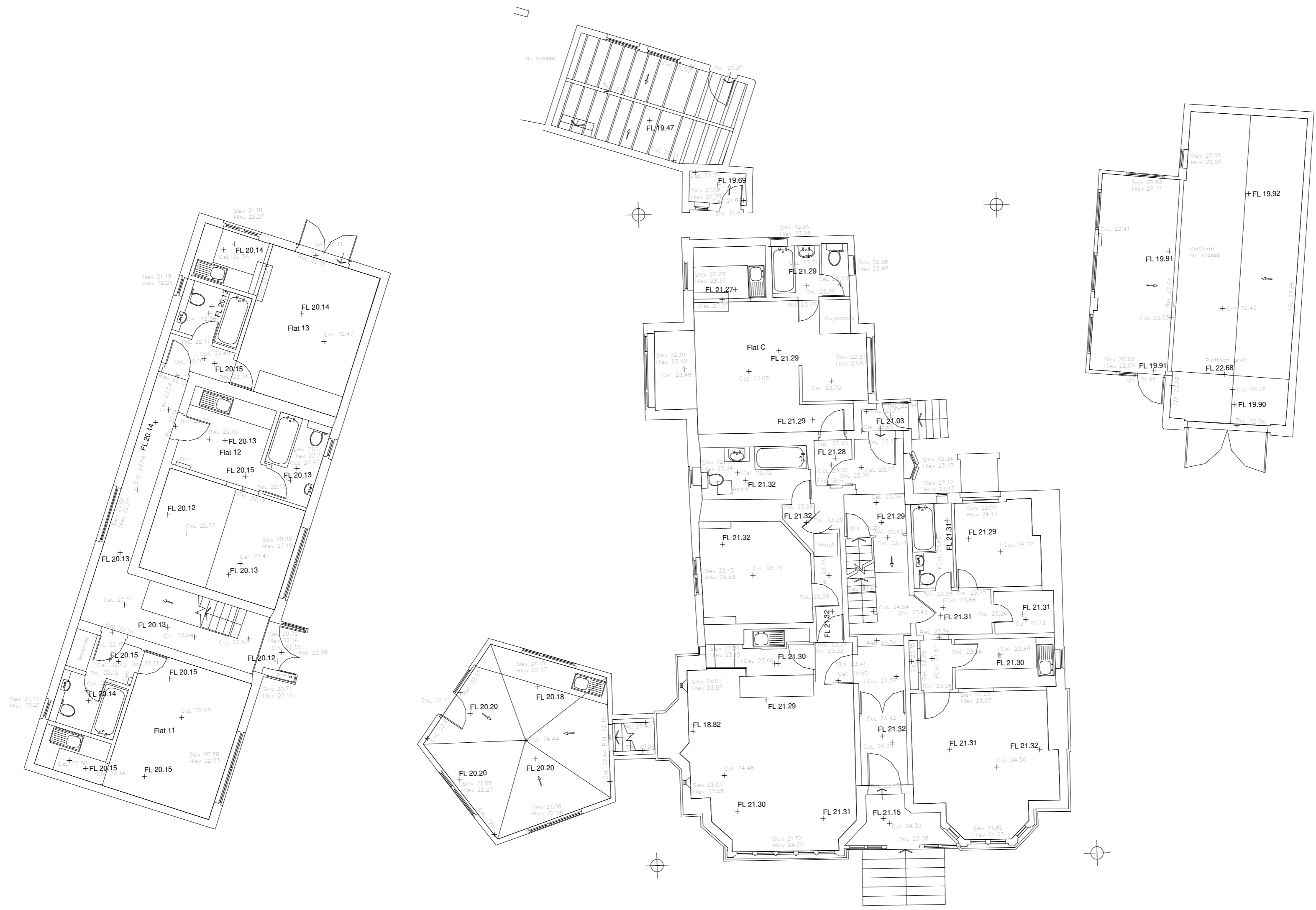
Ground Floor 1:100
