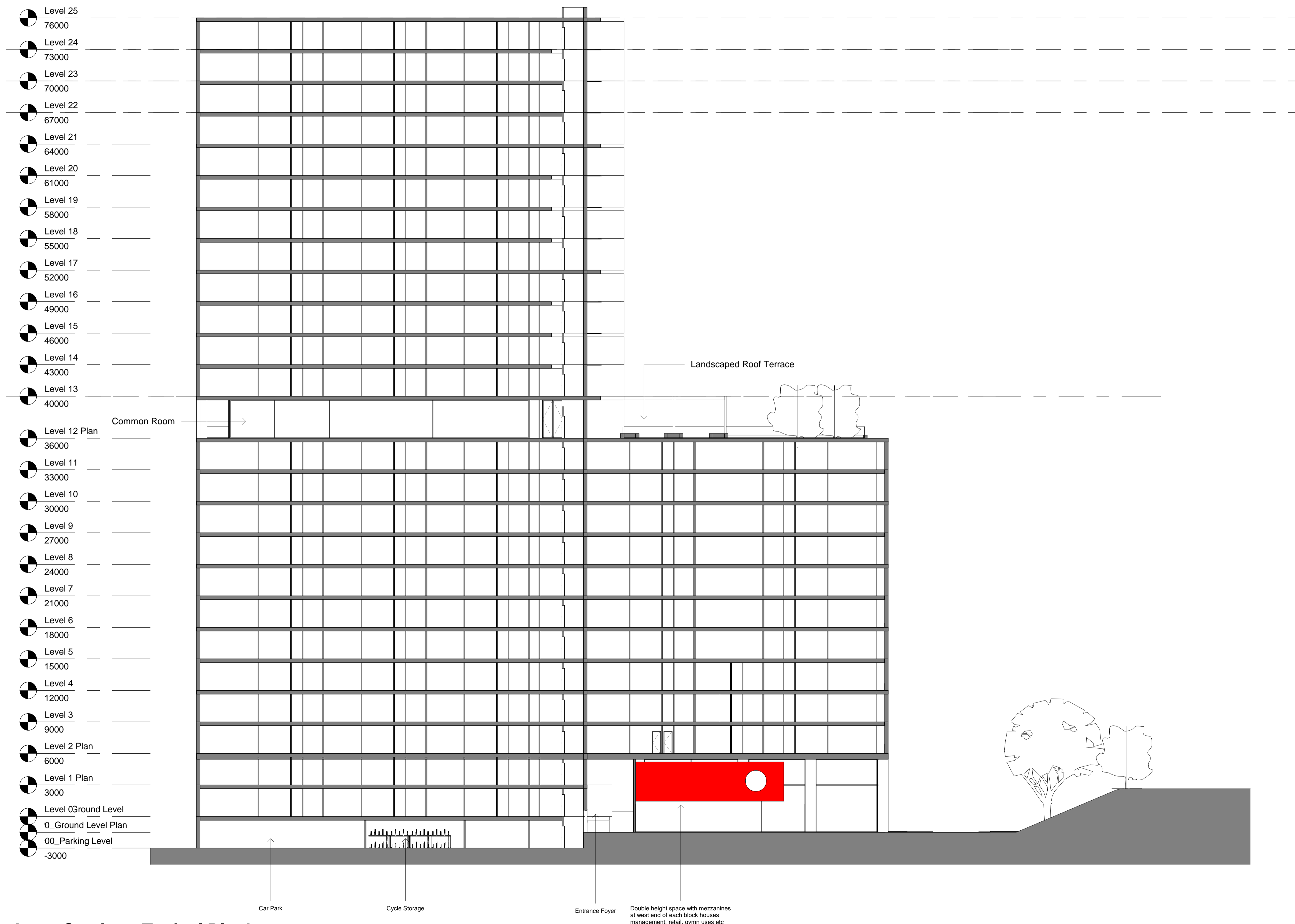
1 Long Section - Typical Block 1 : 200
