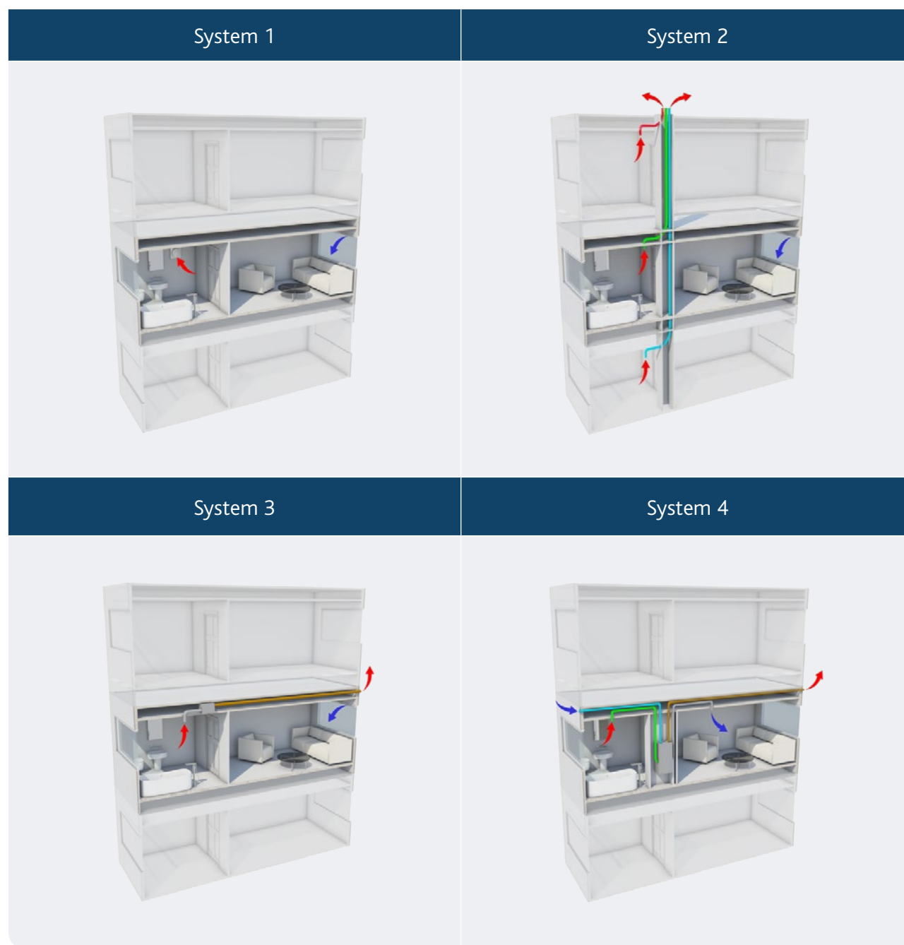
Figure A-1 Illustrations of ADF ventilation systems
